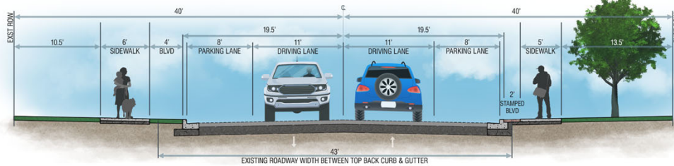
SUNSET DRIVE SOUTH OF I-94 — 14TH STREET NW TO BOUNDARY STREET NW, CONCEPT 1
